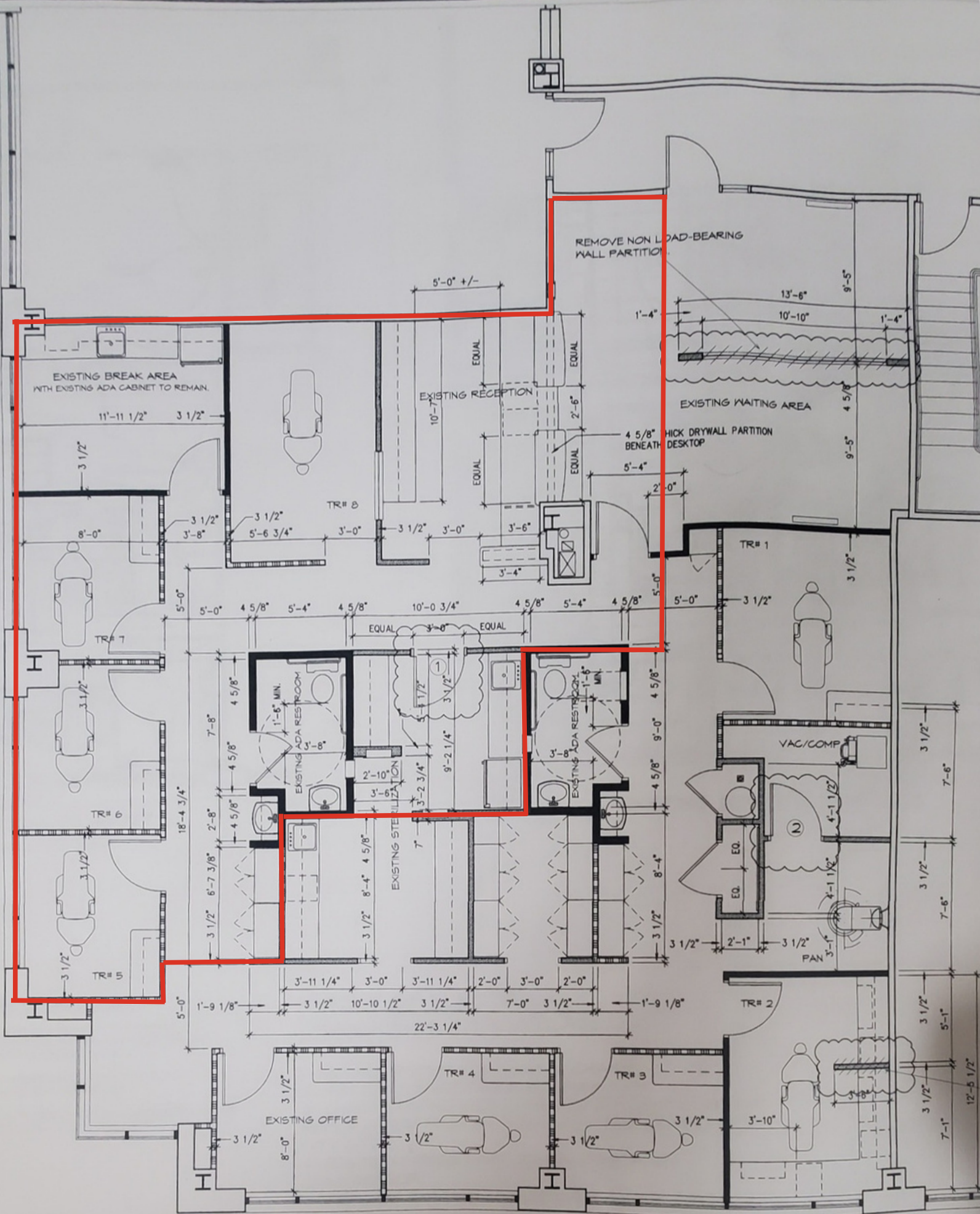
EXISTING FLOOR PLAN 1/4" = 1' 0"
